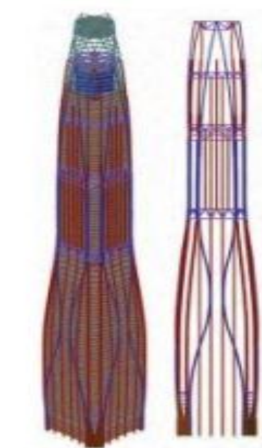
Figure 4. Sloped column system (Source: SOM)
