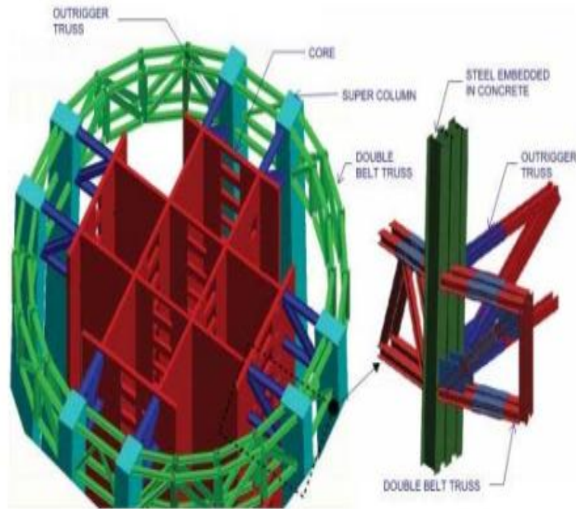
Figure 5. Mega frame for Shanghai Tower and outrigger detail
